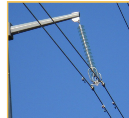
BC Hydro - North Transmission Line (NTL) 287kV twin bundle 325km Line Hardware & fittings and damping system.
